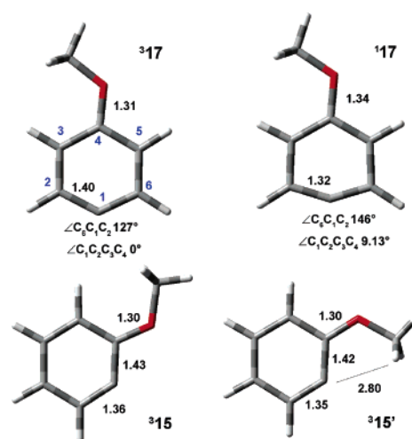
Figure 2. Bond lengths (Å), angles ( \angle , in deg), and dihedral angles ( \angle , in deg) for triplet and singlet 4-methoxyphenyl cation 3 17 and 1 17 and for the two conformers of the triplet 2-methoxyphenyl cation 3 15 and 3 15' as obtained by B3LYP/6-31G(d) calculations in MeCN bulk.
